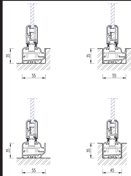
Bottom Track Options
