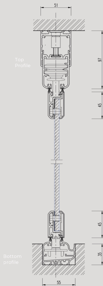
Section Through SF25
